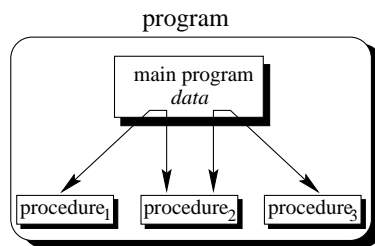
Figure 2.3: Procedural programming. The main program coordinates calls to procedures and hands over appropriate data as parameters.
